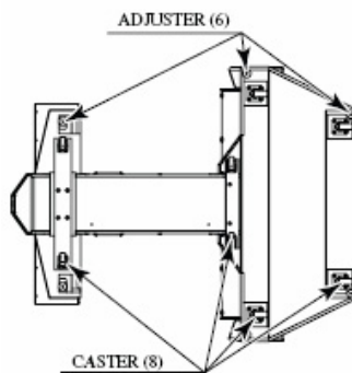
Underside view
