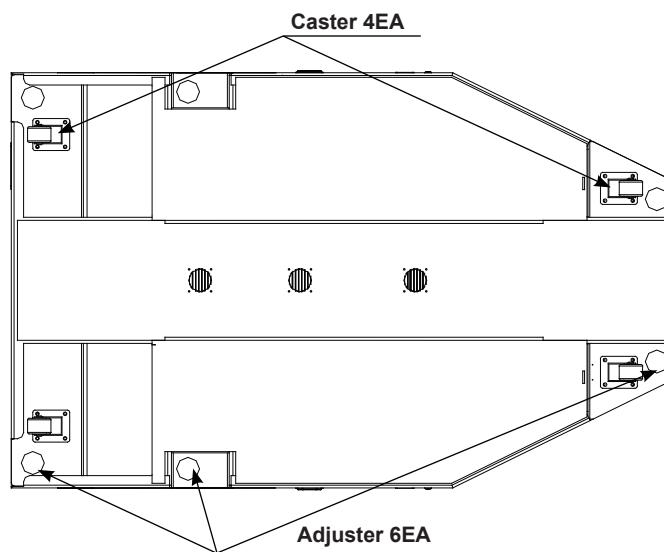
FIG. 6-1a Bottom View
