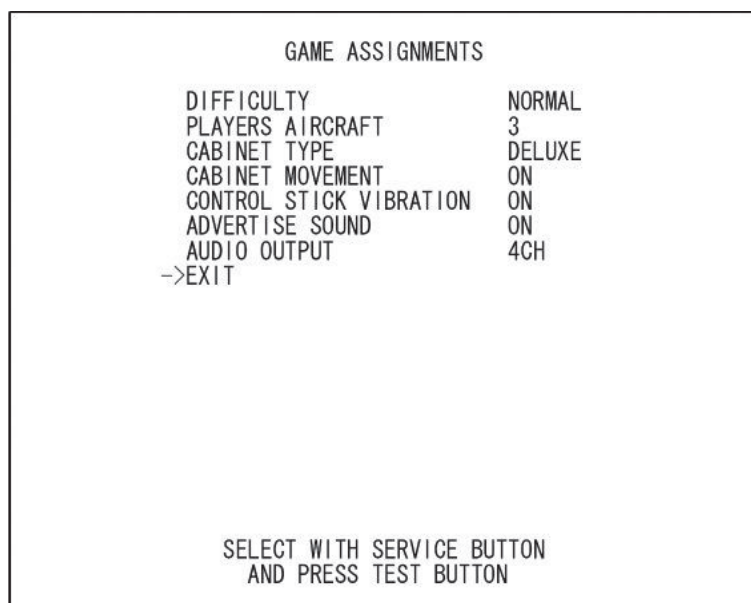
FIG. 9-4c GAME ASSIGNMENTS Screen
