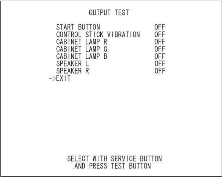
FIG. 9-4b01 OUTPUT TEST Screen (2CH)
