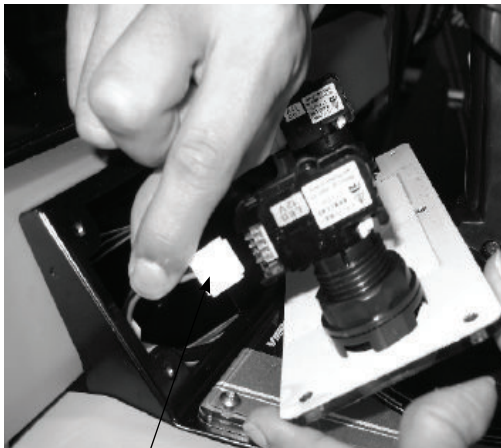
Connector (4P)
