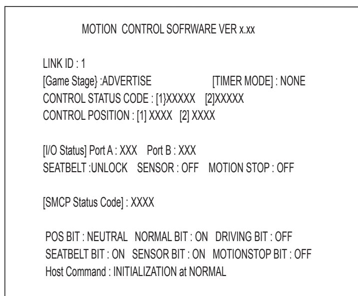
FIG. 9-5 MOTION CONTROL BD STATUS Screen
